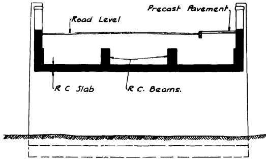
CROSS SECTION UPSTANDING BEAM & SLAB TYPE
